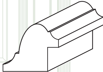
5125-BB 1 3/16" x 1" (1/2" Rabbet) CHE, OAK, POP
