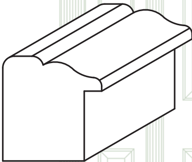
3436-BB 1 1/16" x 1 1/8" (3/4" Rabbet) CHE, FLX, OAK, POP
