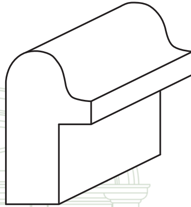
5144-BB 7/8" x 1 1/2" (3/4" Rabbet) CHE, OAK, POP
